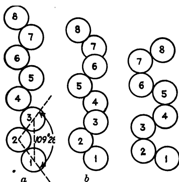
FIG. 6.—Theoretically possible carbon chains. a corresponds to the saturated alcohols. b seems to have no counterpart in aliphatic compounds. c corresponds to the free saturated fatty acids. (Müller and Shearer.)
